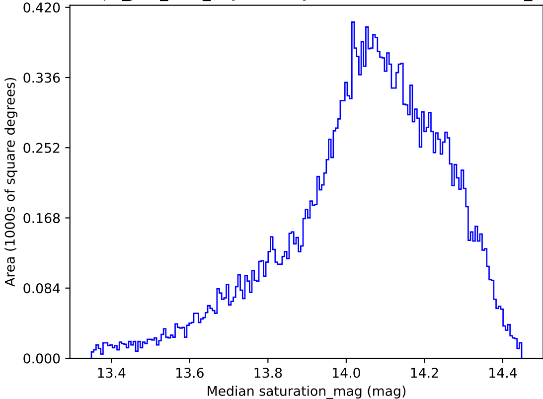
telescope_jerk_v3.5_10yrs All sky z band: Median saturation_mag
