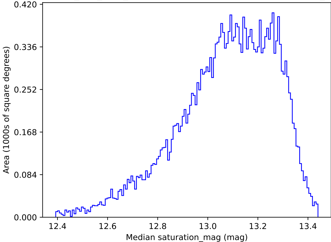
telescope_jerk_v3.5_10yrs All sky y band: Median saturation_mag
