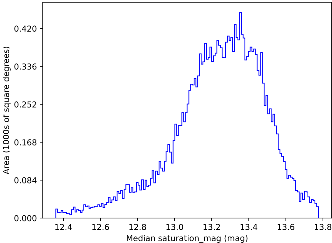
telescope_jerk_v3.5_10yrs All sky u band: Median saturation_mag
