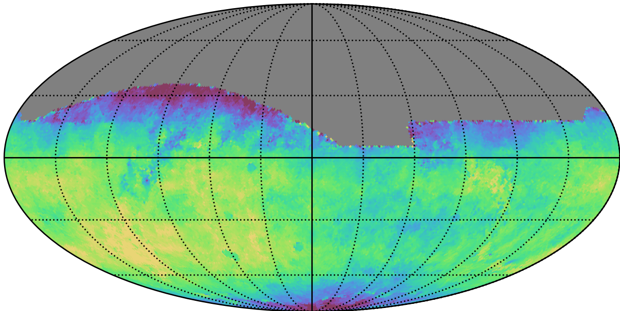
telescope_jerk_v3.5_10yrs All sky i band: Median saturation_mag
