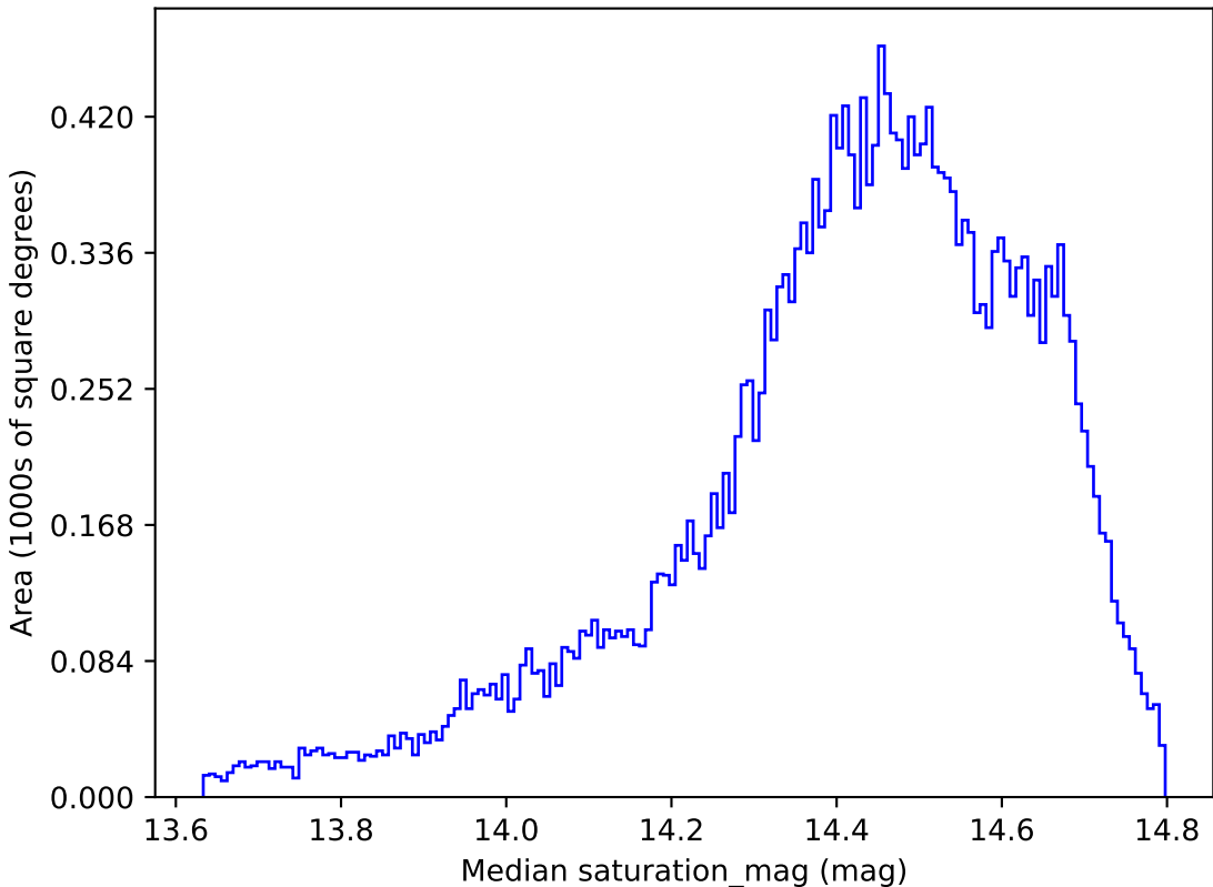
telescope_jerk_v3.5_10yrs All sky i band: Median saturation_mag
