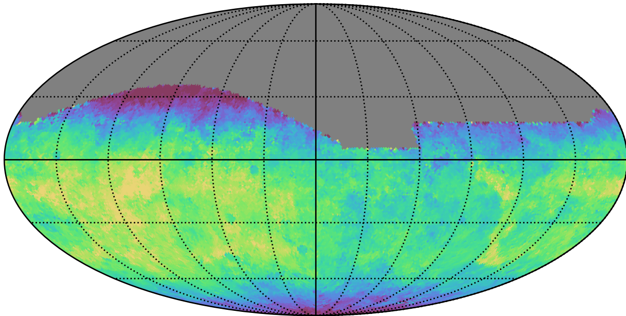
telescope_jerk_v3.5_10yrs All sky g band: Median saturation_mag
