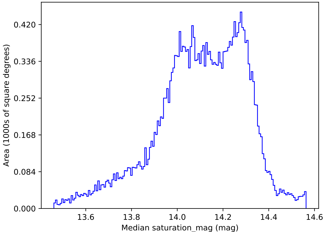
telescope_jerk_v3.5_10yrs All sky all bands: Median saturation_mag
