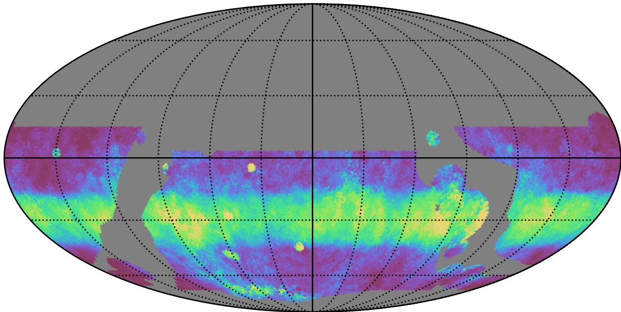
telescope_jerk_v3.5_10yrs WFD y band: Median normairmass
