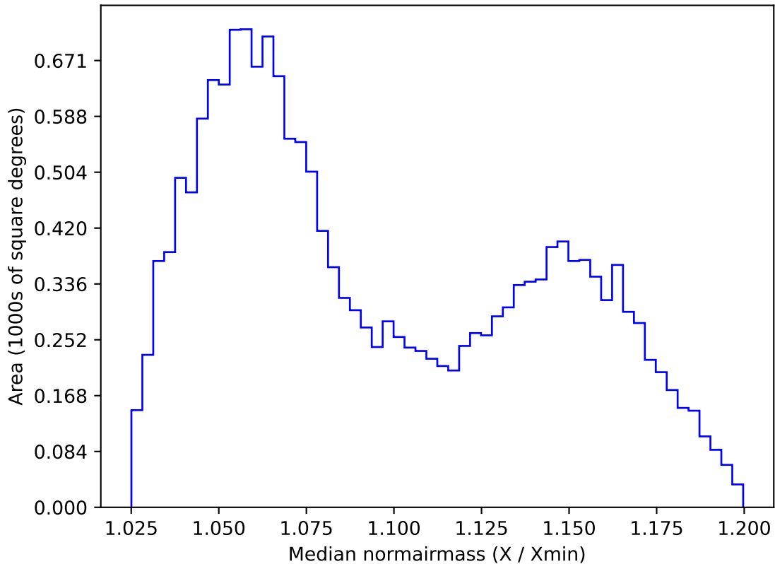
telescope_jerk_v3.5_10yrs WFD y band: Median normairmass
