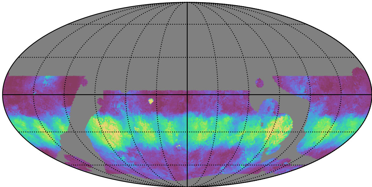
telescope_jerk_v3.5_10yrs WFD u band: Median normairmass
