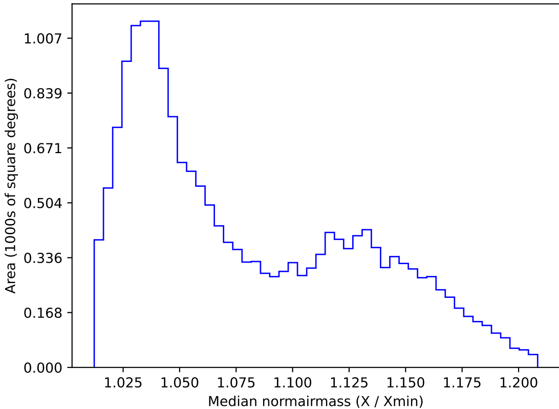
telescope_jerk_v3.5_10yrs WFD u band: Median normairmass
