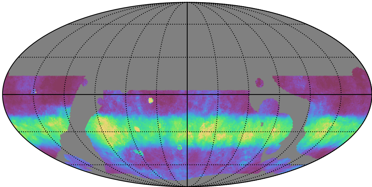
telescope_jerk_v3.5_10yrs WFD r band: Median normairmass
