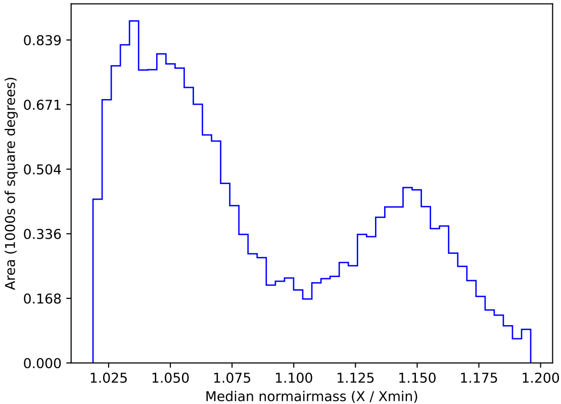
telescope_jerk_v3.5_10yrs WFD r band: Median normairmass
