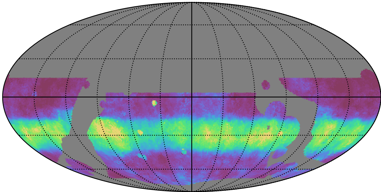
telescope_jerk_v3.5_10yrs WFD i band: Median normairmass
