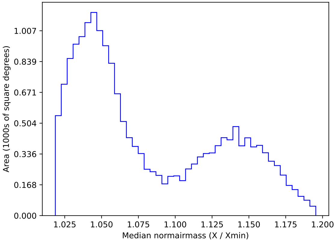
telescope_jerk_v3.5_10yrs WFD i band: Median normairmass
