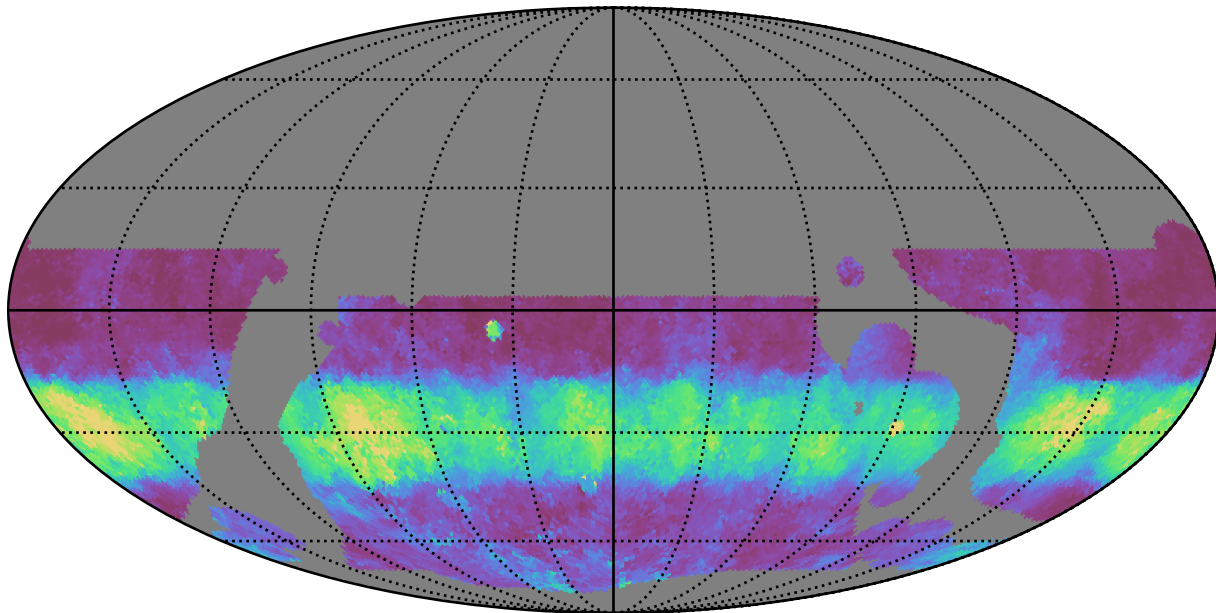
telescope_jerk_v3.5_10yrs WFD g band: Median normairmass
