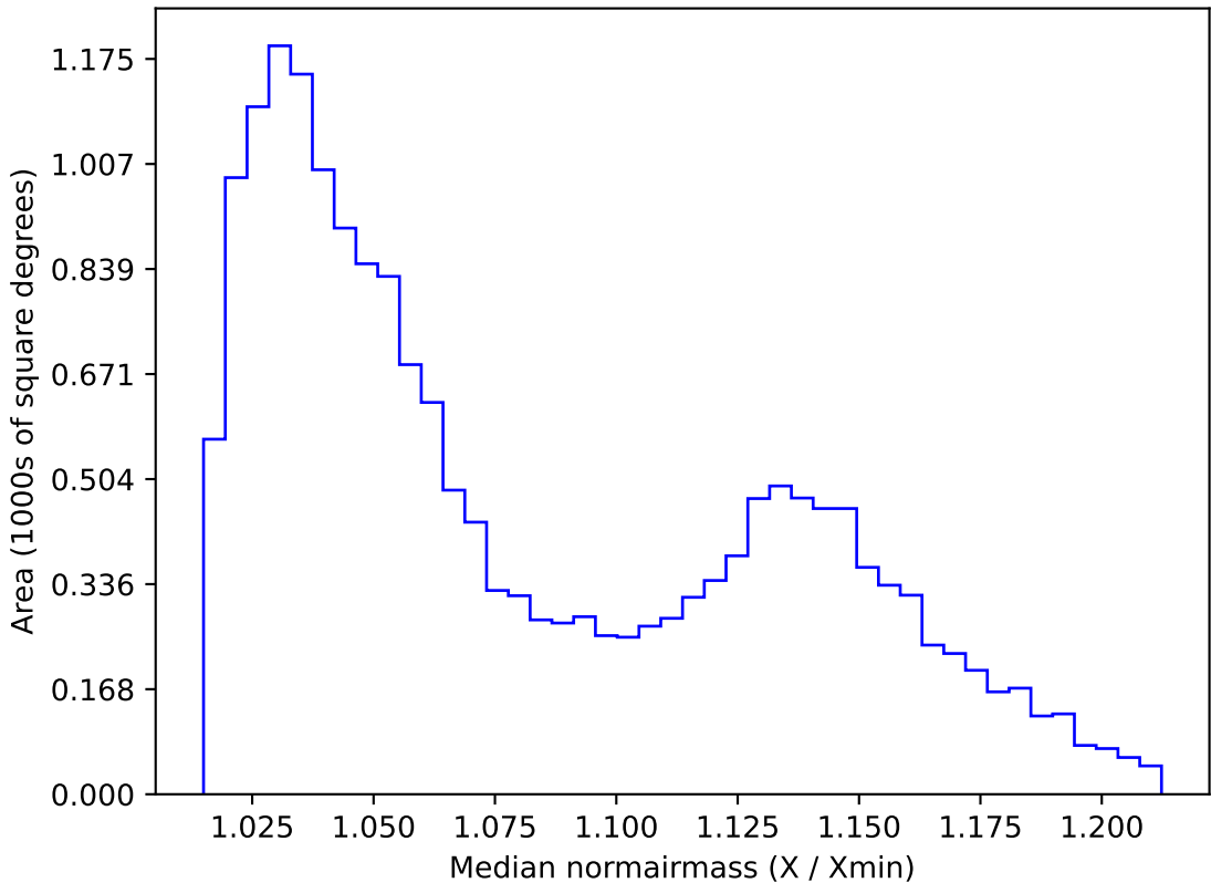
telescope_jerk_v3.5_10yrs WFD g band: Median normairmass
