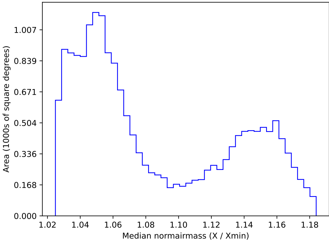
telescope_jerk_v3.5_10yrs WFD all bands: Median normairmass
