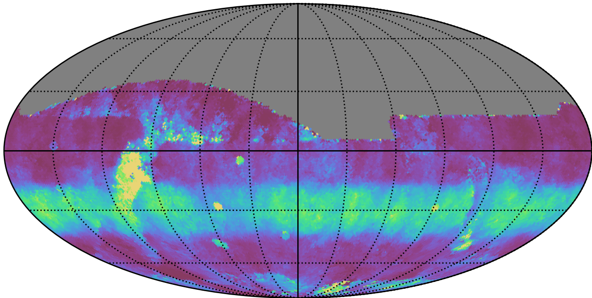
telescope_jerk_v3.5_10yrs All sky z band: Median normairmass
