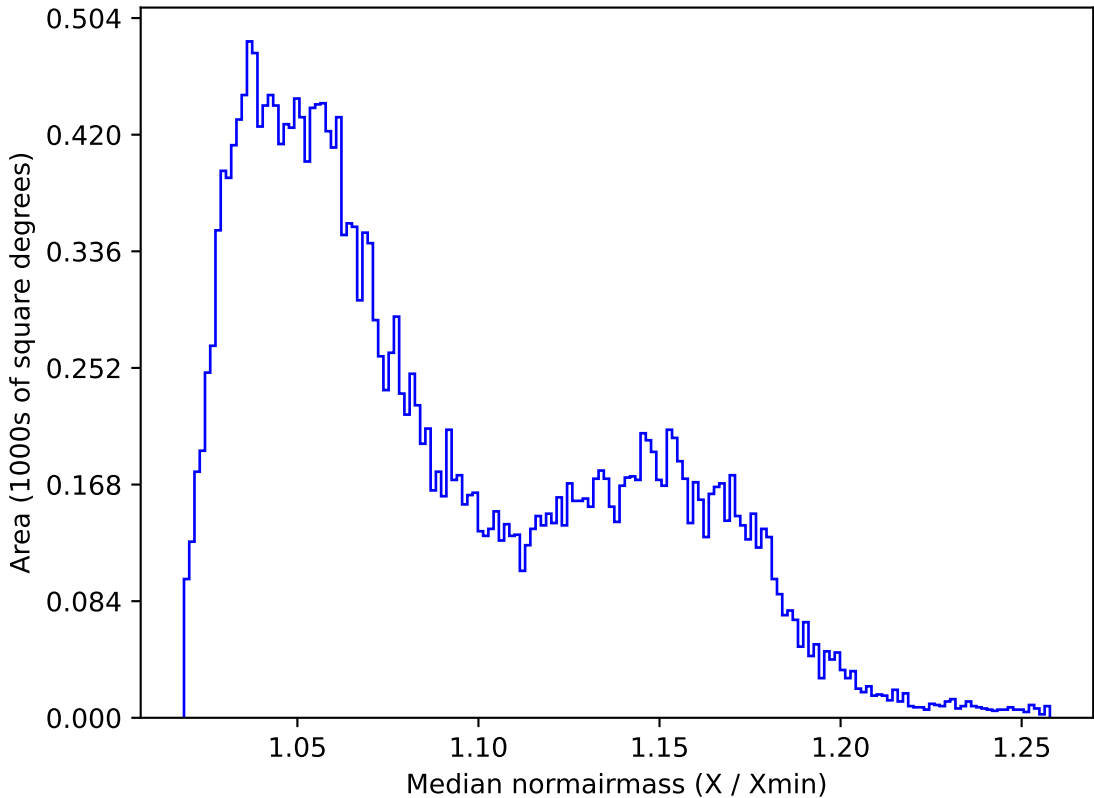
telescope_jerk_v3.5_10yrs All sky z band: Median normairmass
