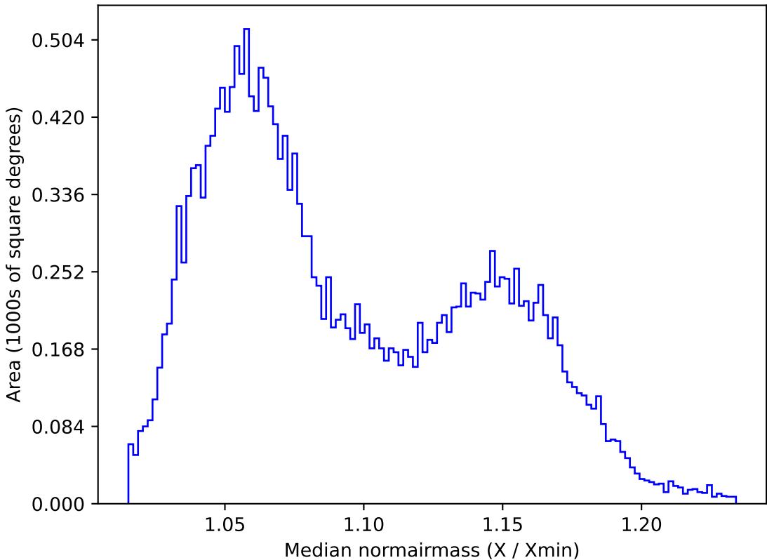
telescope_jerk_v3.5_10yrs All sky y band: Median normairmass
