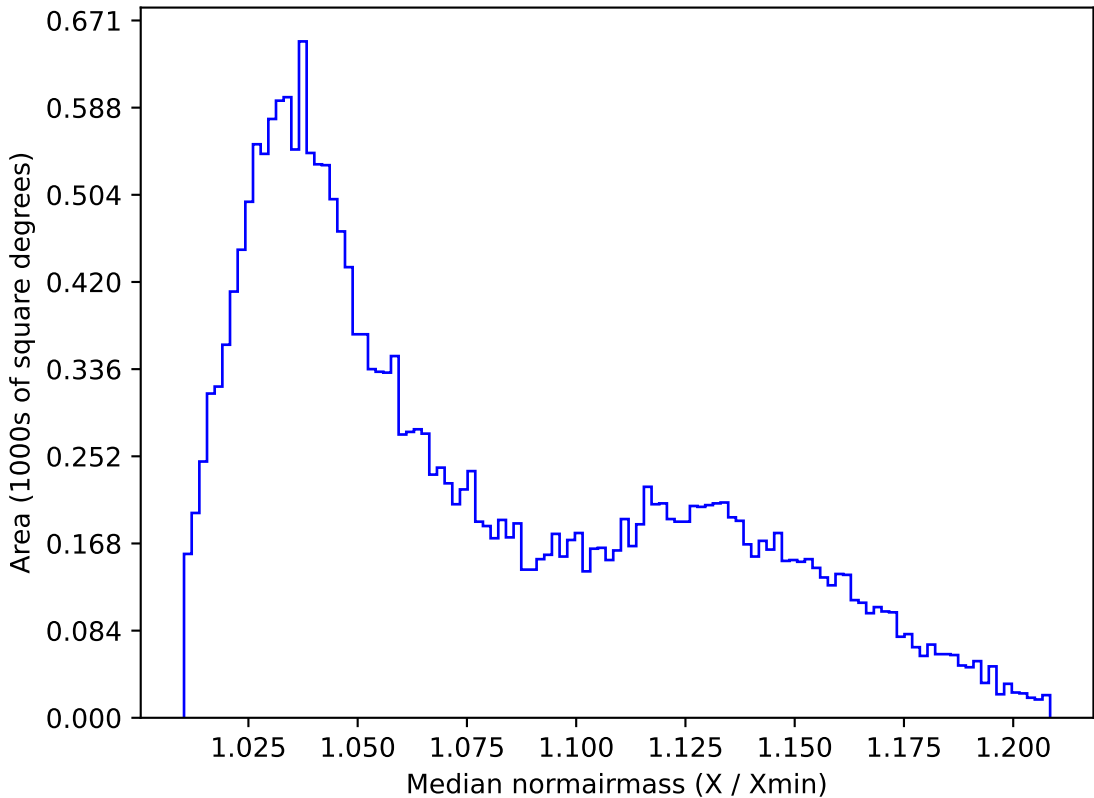
telescope_jerk_v3.5_10yrs All sky u band: Median normairmass
