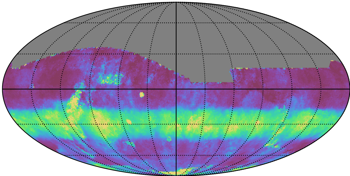
telescope_jerk_v3.5_10yrs All sky r band: Median normairmass
