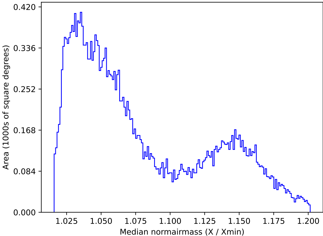
telescope_jerk_v3.5_10yrs All sky r band: Median normairmass
