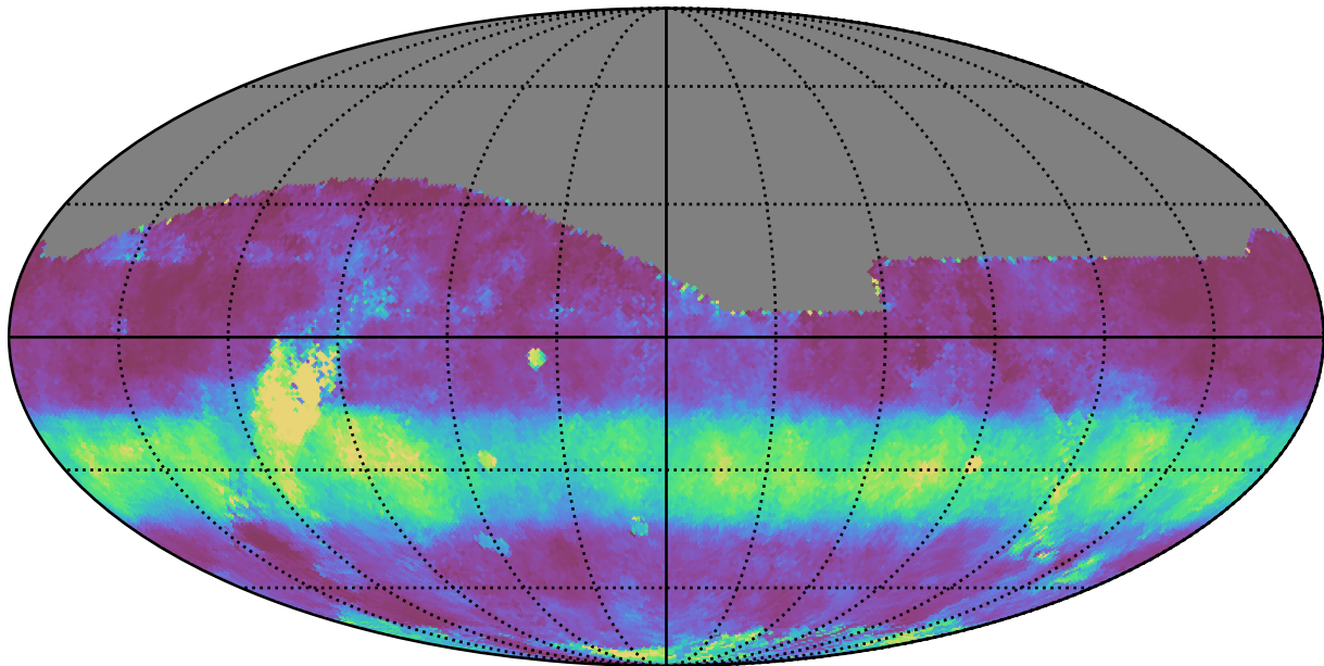
telescope_jerk_v3.5_10yrs All sky i band: Median normairmass
