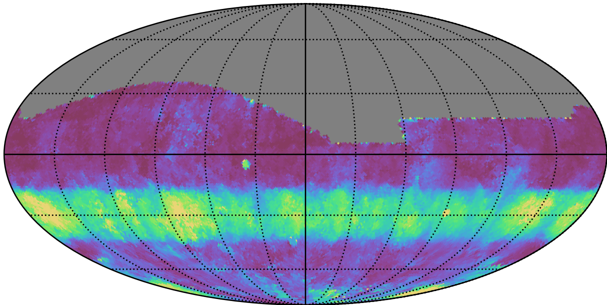
telescope_jerk_v3.5_10yrs All sky g band: Median normairmass
