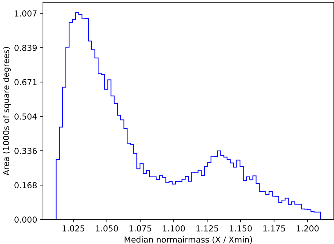
telescope_jerk_v3.5_10yrs All sky g band: Median normairmass
