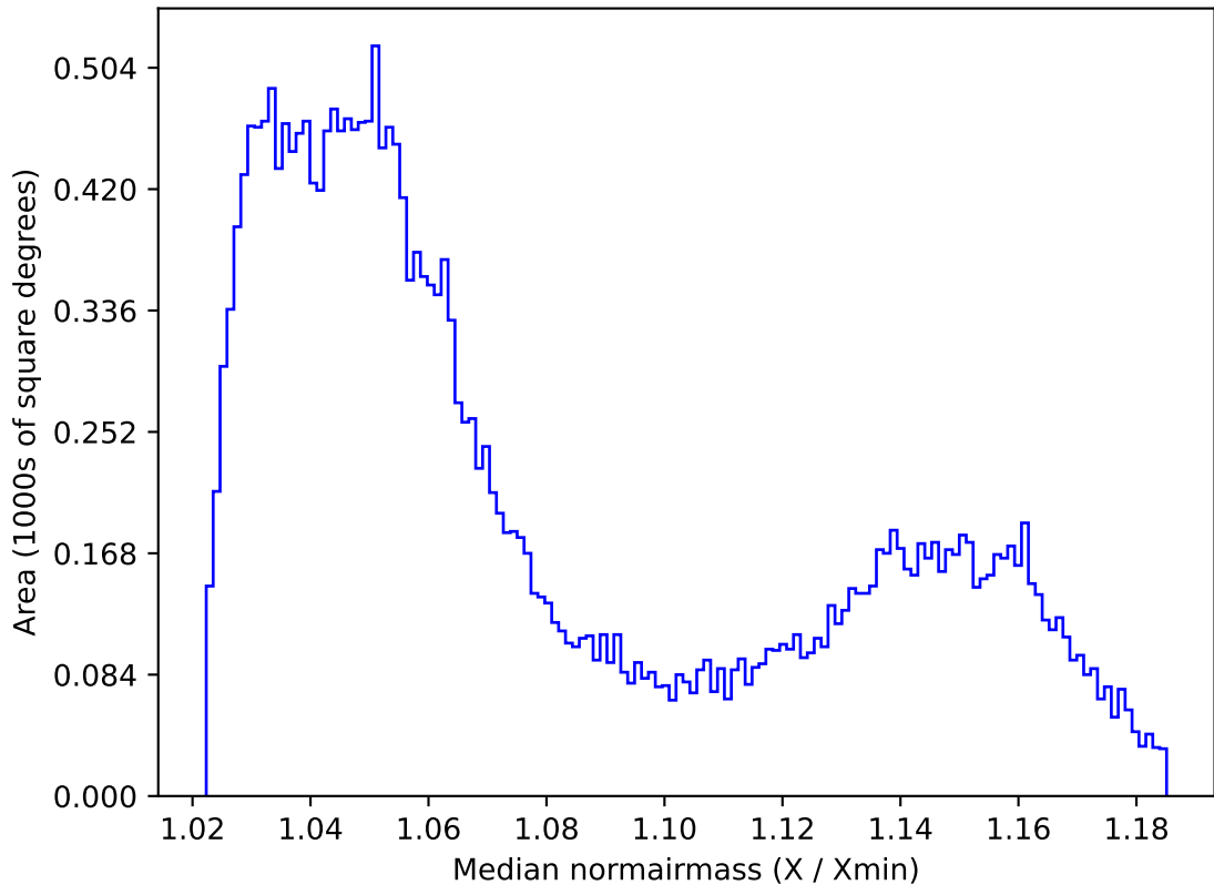
telescope_jerk_v3.5_10yrs All sky all bands: Median normairmass
