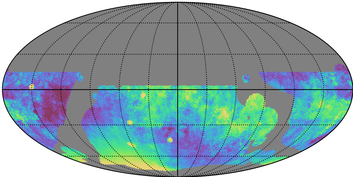
telescope_jerk_v3.5_10yrs WFD z band: Median moonDistance
