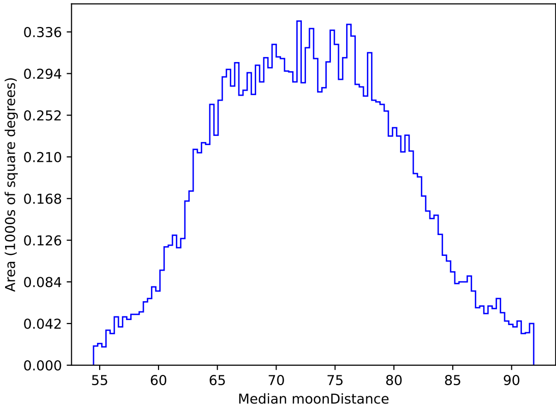
telescope_jerk_v3.5_10yrs WFD z band: Median moonDistance
