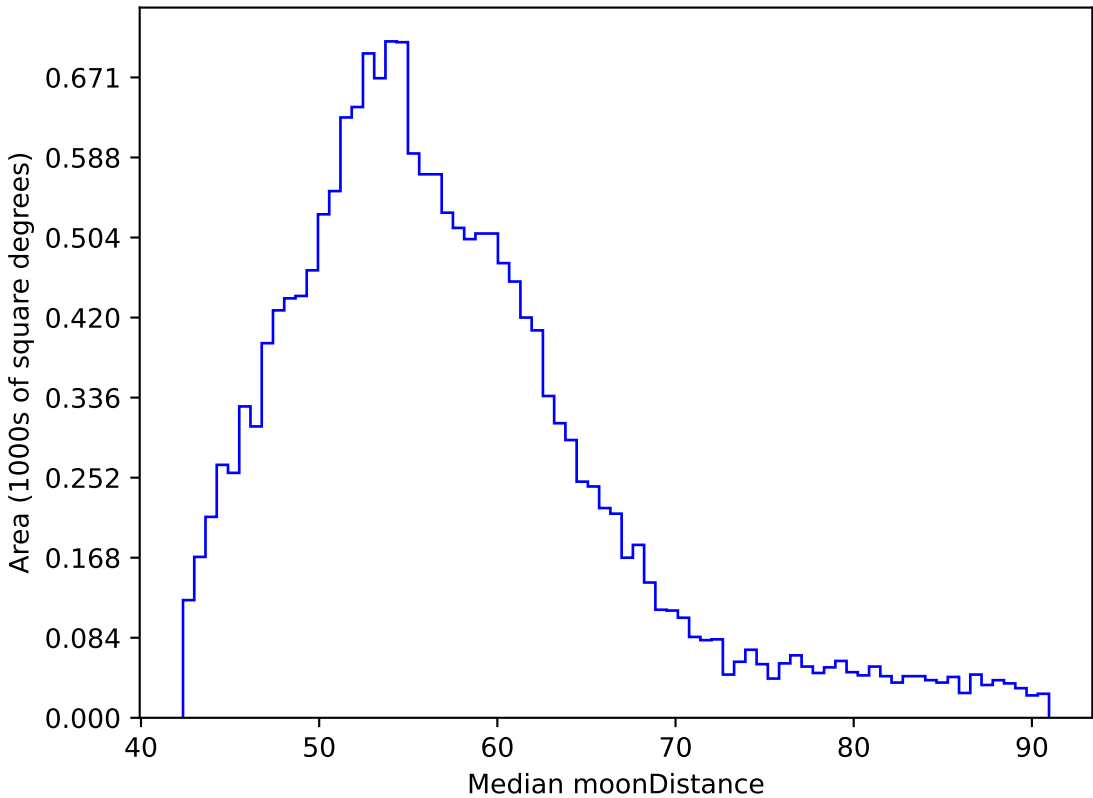
telescope_jerk_v3.5_10yrs WFD y band: Median moonDistance
