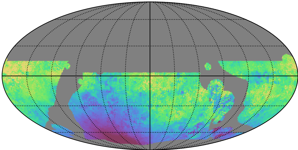
telescope_jerk_v3.5_10yrs WFD u band: Median moonDistance
