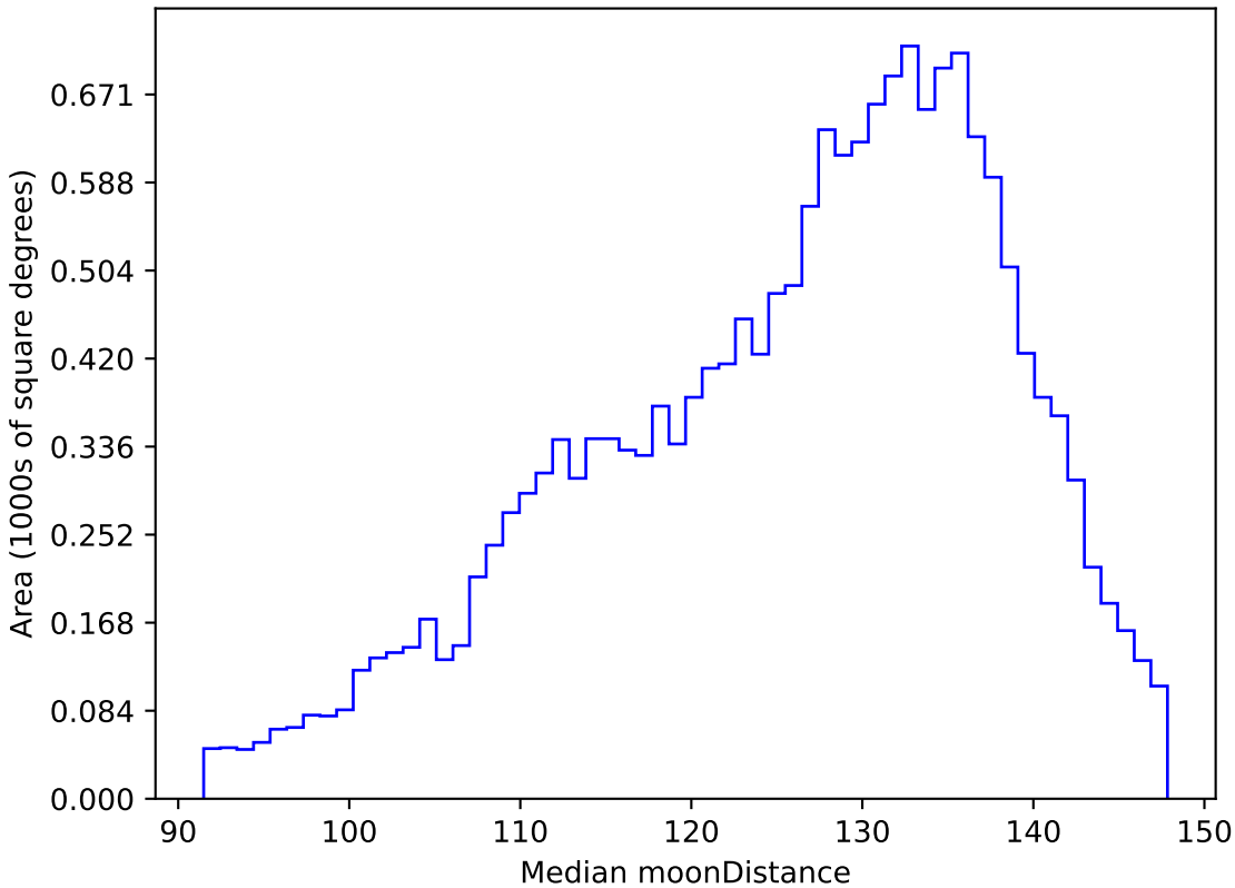
telescope_jerk_v3.5_10yrs WFD u band: Median moonDistance
