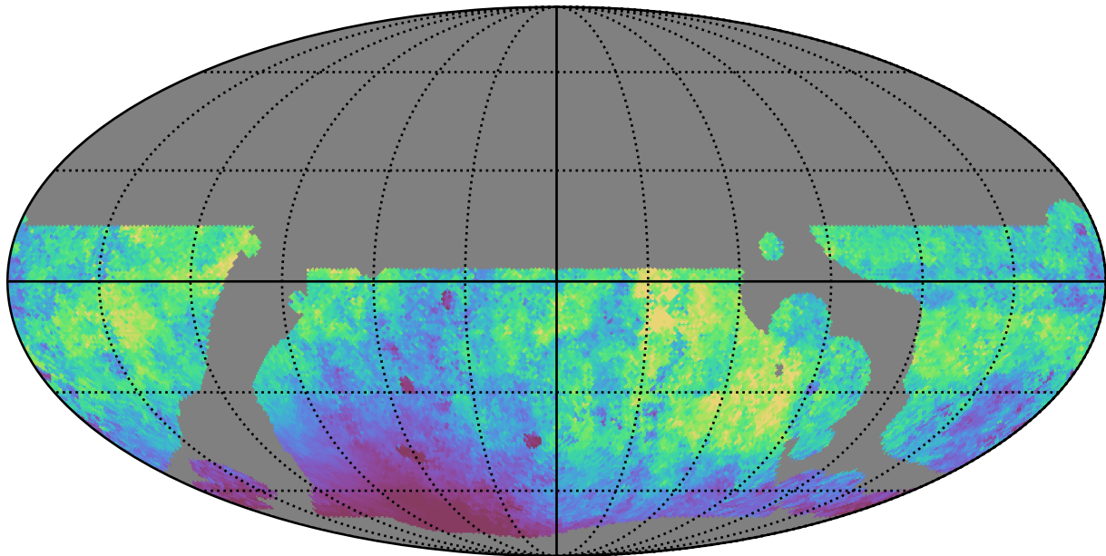
telescope_jerk_v3.5_10yrs WFD r band: Median moonDistance
