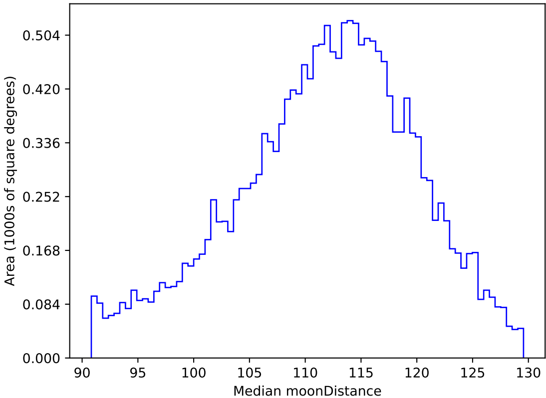
telescope_jerk_v3.5_10yrs WFD r band: Median moonDistance
