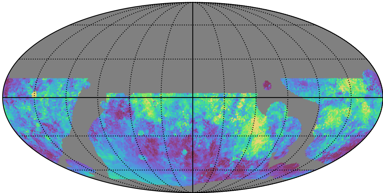
telescope_jerk_v3.5_10yrs WFD i band: Median moonDistance
