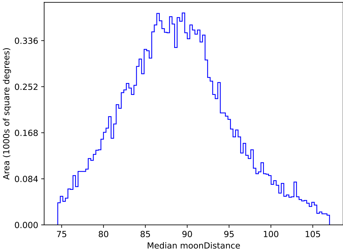
telescope_jerk_v3.5_10yrs WFD i band: Median moonDistance
