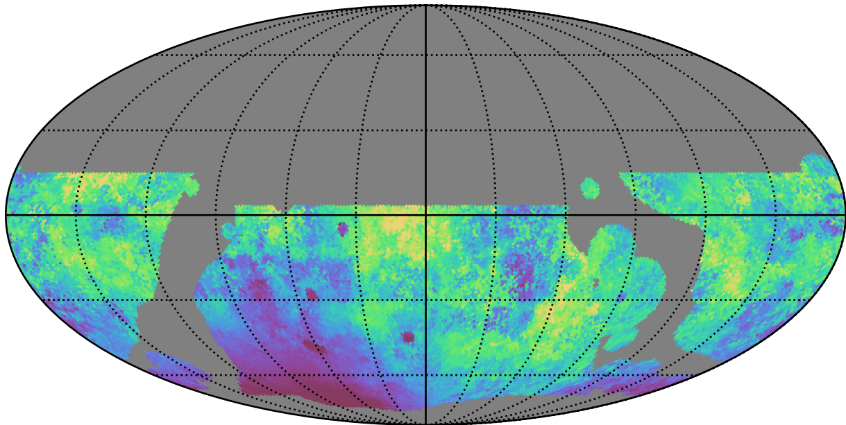
telescope_jerk_v3.5_10yrs WFD g band: Median moonDistance
