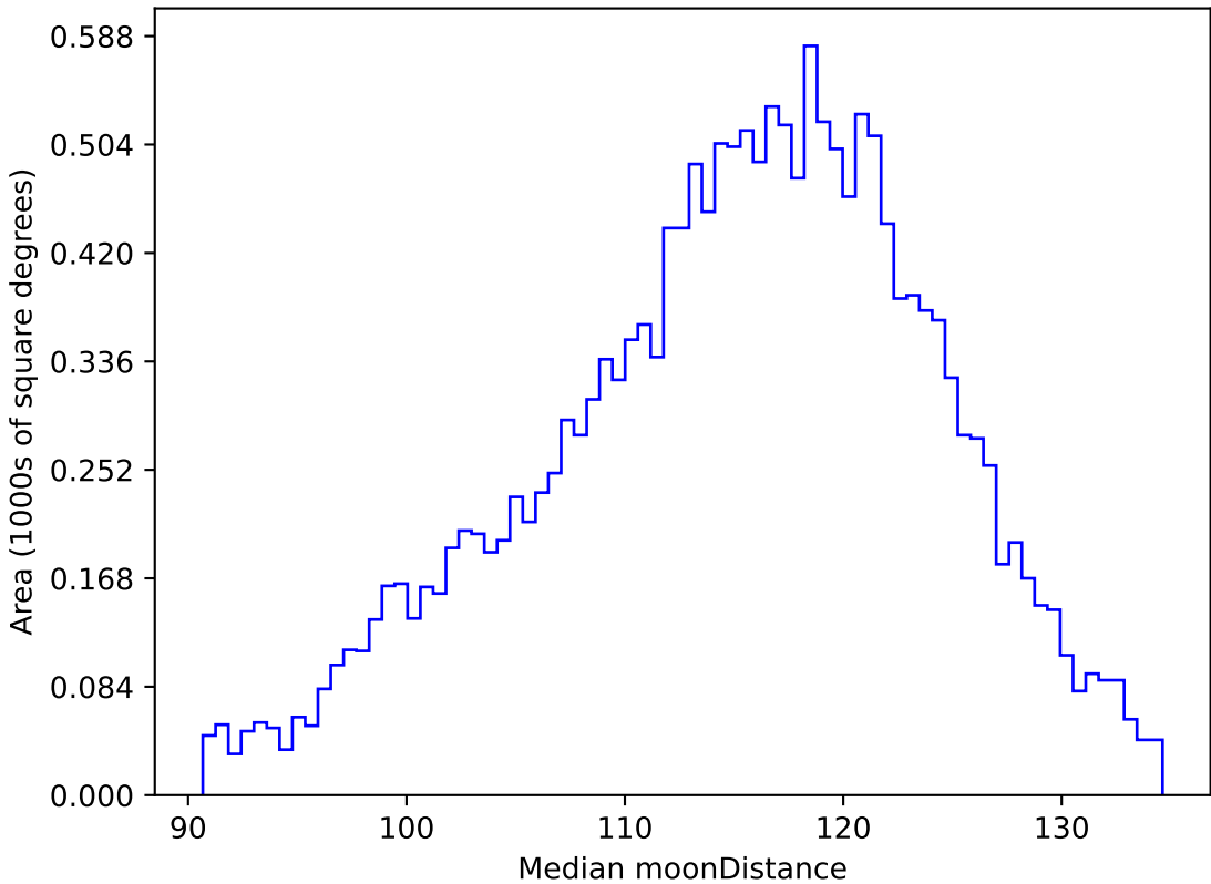
telescope_jerk_v3.5_10yrs WFD g band: Median moonDistance
