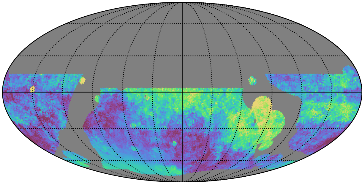
telescope_jerk_v3.5_10yrs WFD all bands: Median moonDistance
