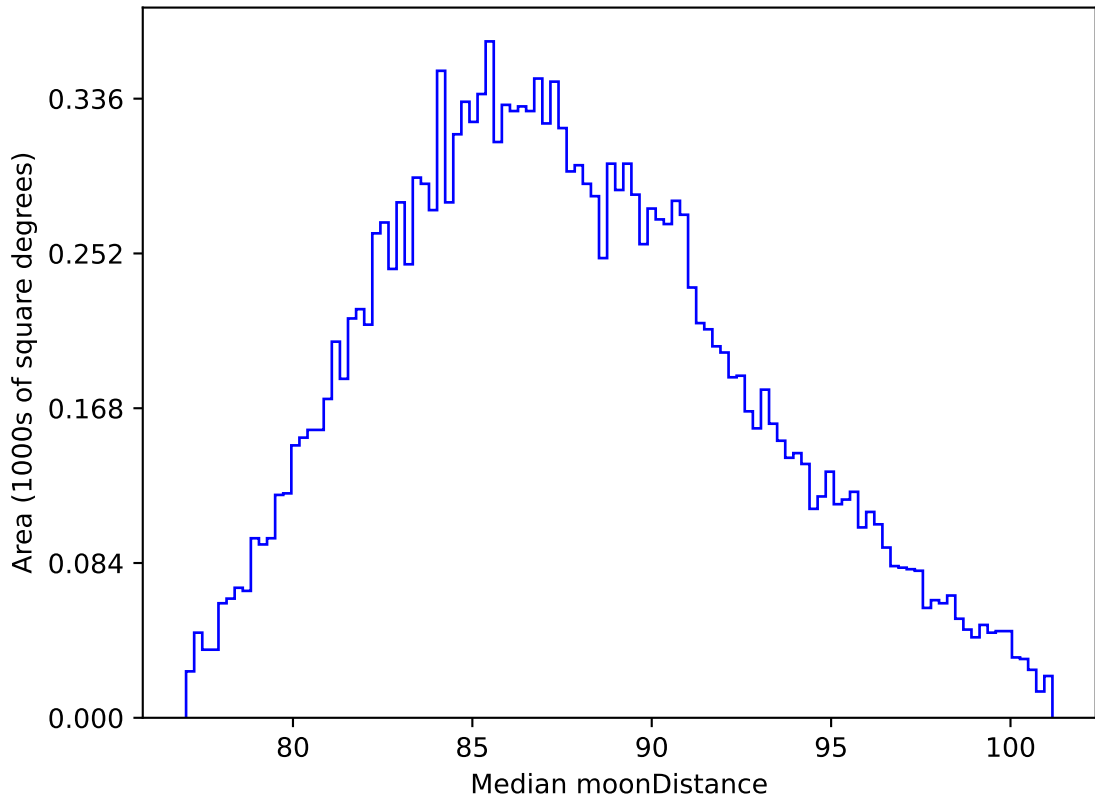
telescope_jerk_v3.5_10yrs WFD all bands: Median moonDistance
