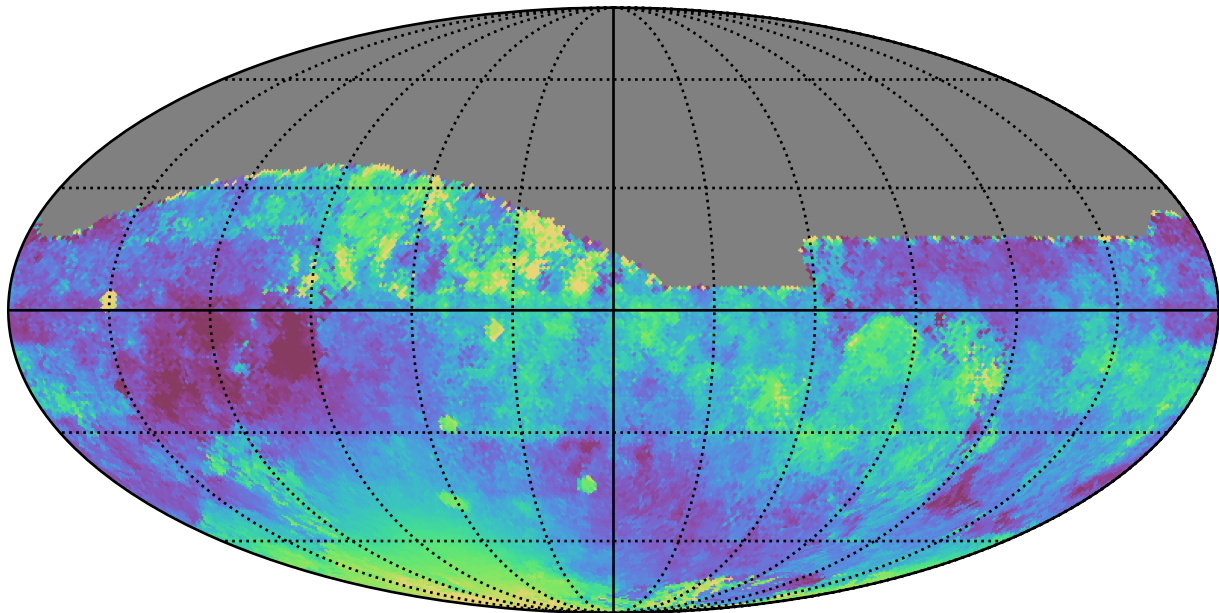
telescope_jerk_v3.5_10yrs All sky z band: Median moonDistance
