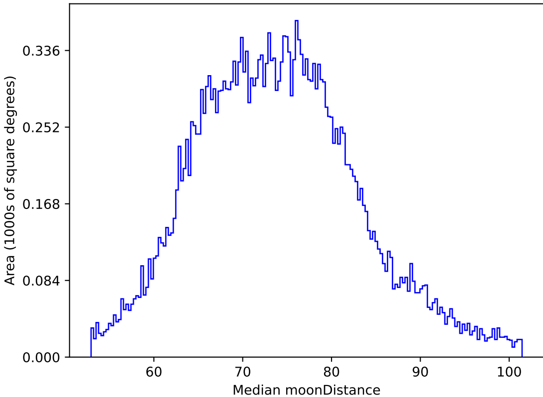
telescope_jerk_v3.5_10yrs All sky z band: Median moonDistance
