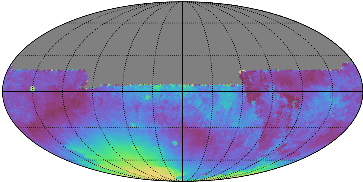
telescope_jerk_v3.5_10yrs All sky y band: Median moonDistance
