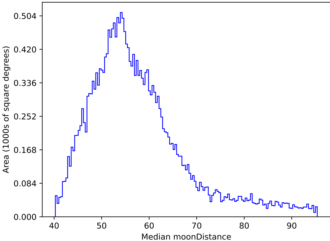
telescope_jerk_v3.5_10yrs All sky y band: Median moonDistance
