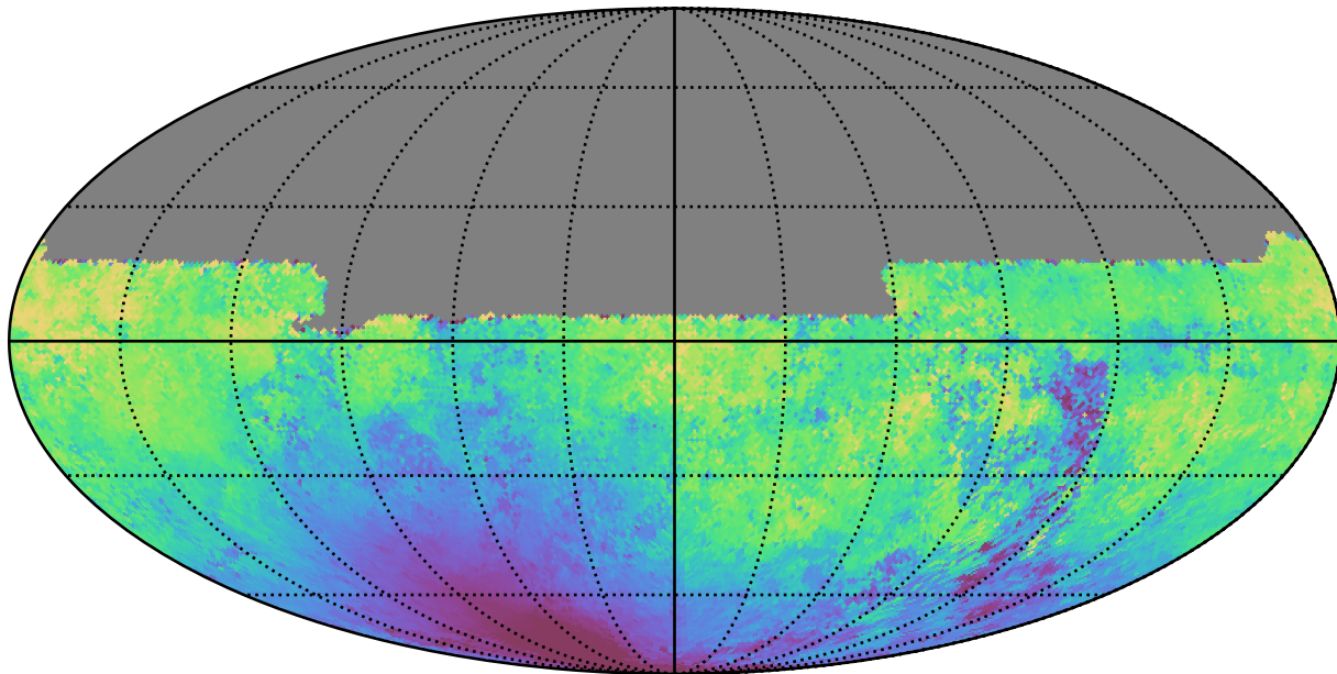
telescope_jerk_v3.5_10yrs All sky u band: Median moonDistance
