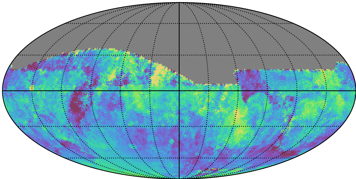
telescope_jerk_v3.5_10yrs All sky i band: Median moonDistance
