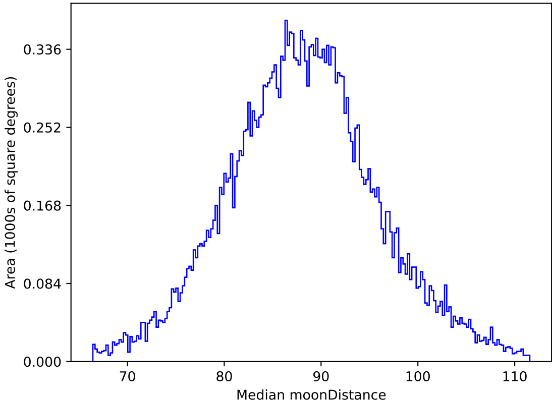
telescope_jerk_v3.5_10yrs All sky i band: Median moonDistance
