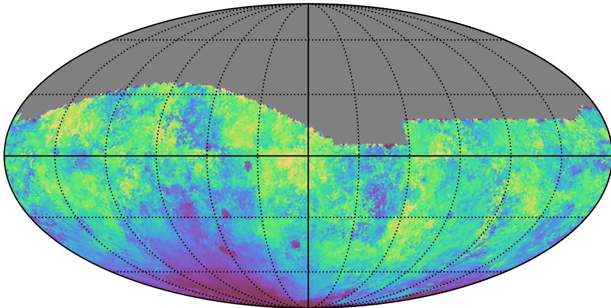
telescope_jerk_v3.5_10yrs All sky g band: Median moonDistance
