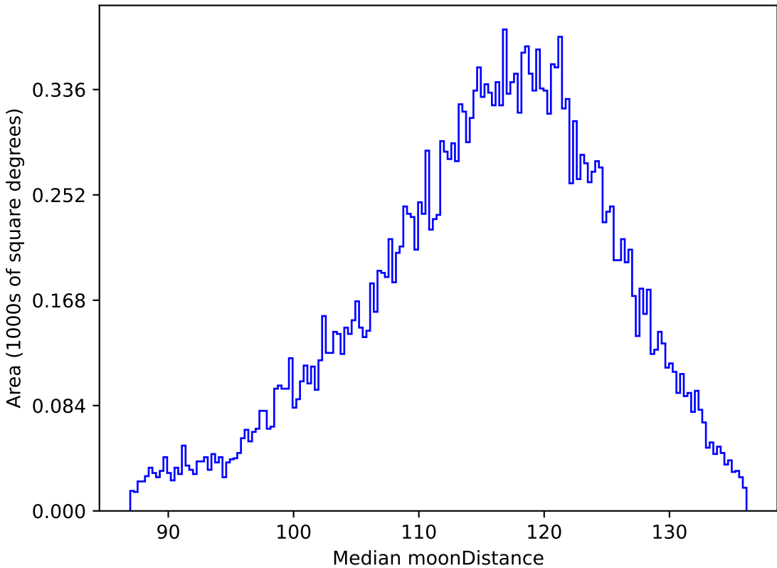
telescope_jerk_v3.5_10yrs All sky g band: Median moonDistance
